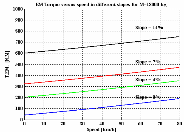
Fig. 4 EM Torque versus vehicle speed on the different slopes
