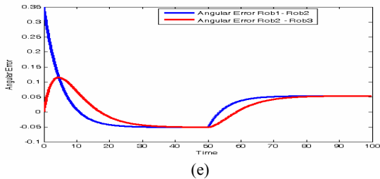
Fig. 7 Leader Robot goes on reference path that has initially its curvature equal to -0.05 and change the curvature to 0.05 at time equal to 50s
