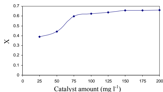
Fig. 4 Effect of catalyst loading on the degree of photodegradation of diazinon. [diazinon] 0 = 20 mg l -1 ; pH neutral; irradiation time = 50 min
