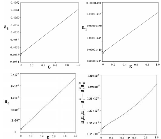
Fig. 1 The parameter space for the endemic equilibrium point which satisfies the Routh-Hurwitz criteria. The values of the other parameters are \mu_H = 0.000039139 \text{ day}^{-1} ,
