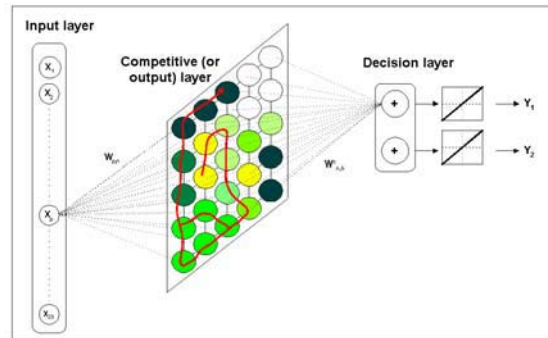
Figure 1: From left to right, the first two layers represent the general architecture of the Self Organizing Map (SOM): Xi(i=1...23) input corresponds to the percentage of the power spectrum of I band (PSSi). Wpn(p=1...23, n=1...25) weights from input to competitive layer. The other two layers indicate the principle of Learning Vector Quantization (LVQ)
