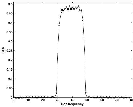
Fig. 4 Performance of HV2 packets
