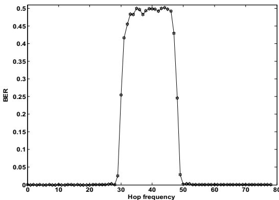
Fig. 5 Performance of HV3 packets
