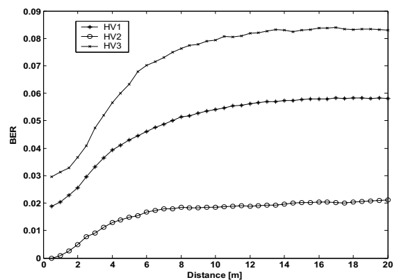
Fig. 7. BER versus distance between the master and the slave
