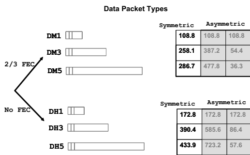
Fig.2 Structure of the Data Packets
