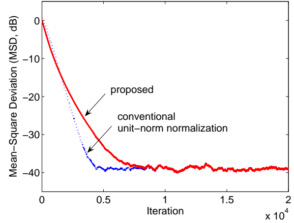
Fig. 1. Performance of two adaptive algorithms in constrained mean-square optimization (conventional vs. proposed)
