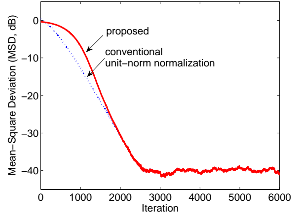
Fig. 3. Performance of two adaptive algorithms in PCA (conventional vs. proposed method)
