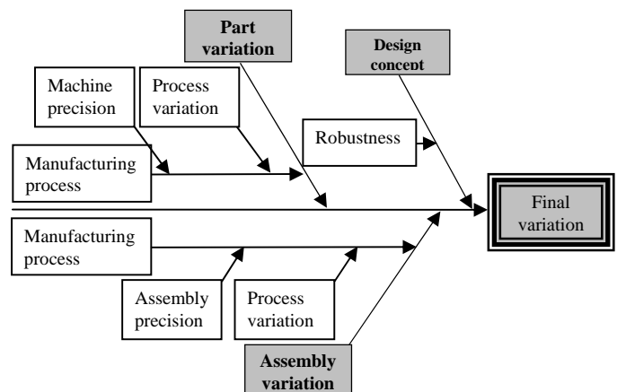
Fig. 1 Geometrical variation contributors, process industry [13]
