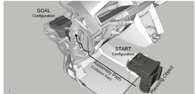
Fig. 1 A typical application of rigid-body path planning at Volvo Car Corporation. Engineer input consists of choosing planning object along with setting its start and goal configurations. A collision-free path, if in existence, is automatically determined
