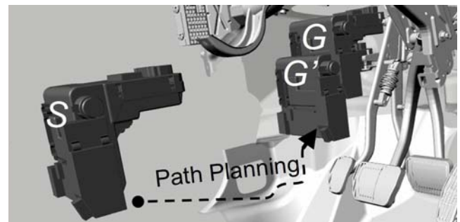
Fig. 4 Whereas path planning is conducted between S and G' , the feasibility between G' and G is left for the engineer to manually estimate. The distance between G and G' is heavily exaggerated for graphical purposes
