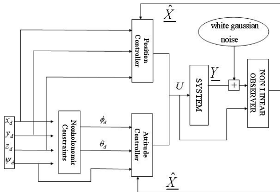
Fig. 2 Synoptic scheme of the proposed controller
