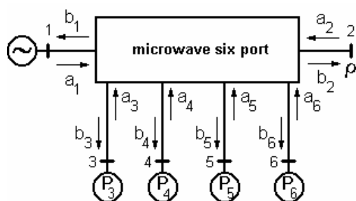
Fig. 1. Basic arrangement of the six-port.
