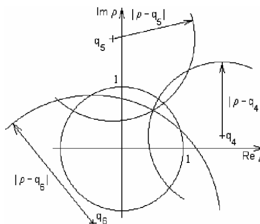
Fig. 2. Geometrical interpretation of the formulas in [1].
