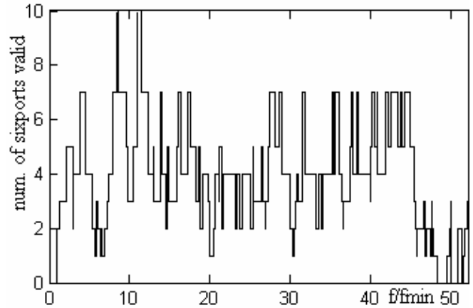
Fig. 4. Example of the multisixport computed for n=5 and \alpha_{\min}=45^\circ .
