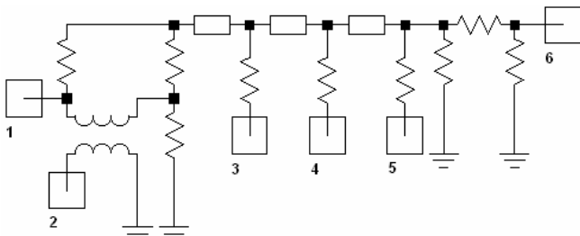
Fig. 3. Design of the simple six-port.
