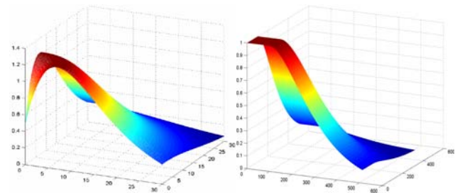
Fig. 5 CSF function models: Mannos (left), Daly (right)
