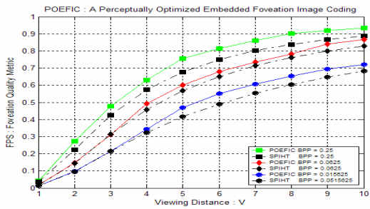
Fig. 8 Foveation Wavelet Quality Index FQWI of POEFIC vs SPIHT BOAT image at 0.015625 bpp, 0.0625 bpp and 0.25 bpp.
