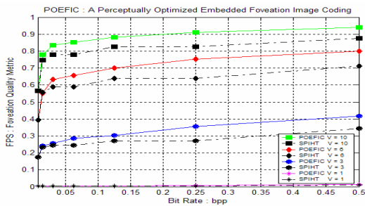
Fig. 7 Foveation Wavelet Quality Index of POEFIC vs SPIHT Mandrill
