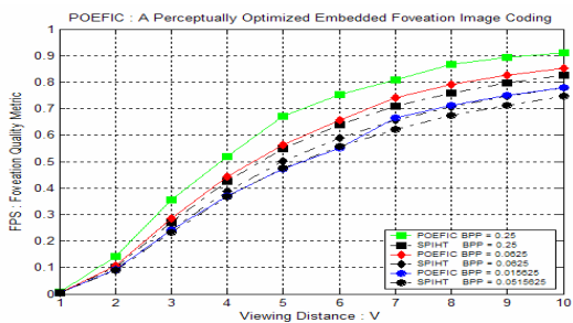
Fig. 9 Foveation Wavelet Quality Index FQWI of POEFIC vs SPIHT Mandrill image at 0.015625 bpp, 0.0625 bpp and 0.25 bpp.
