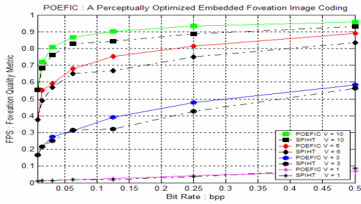
Fig. 6 Foveation Wavelet Quality Index of POEFIC vs SPIHT BOAT
