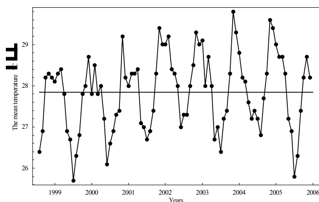
Fig. 2 The mean temperature at Samui Islands from 1999–2006
