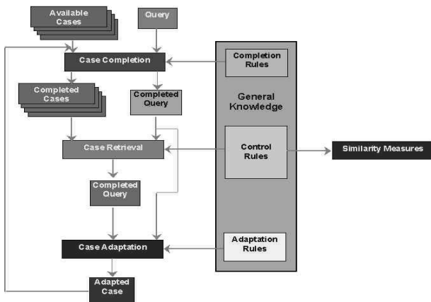
Fig. 4 Incorporating GK rules using CBR
