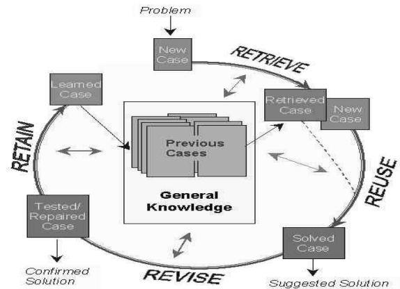
Fig. 3 CBR cycle
