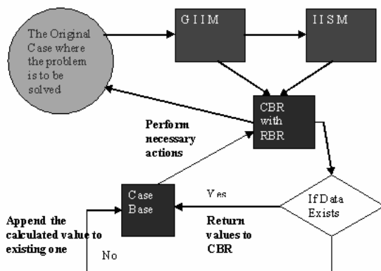
Fig. 5 The Implementation of the system
