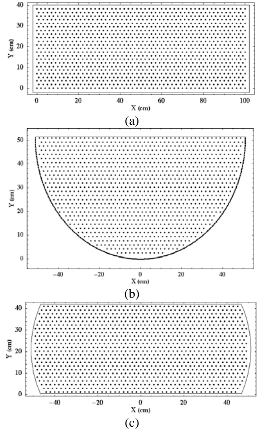
Fig. 1 Configuration of 1162 water particles in three cavities: rectangular, half-circular and beer bucket shapes
