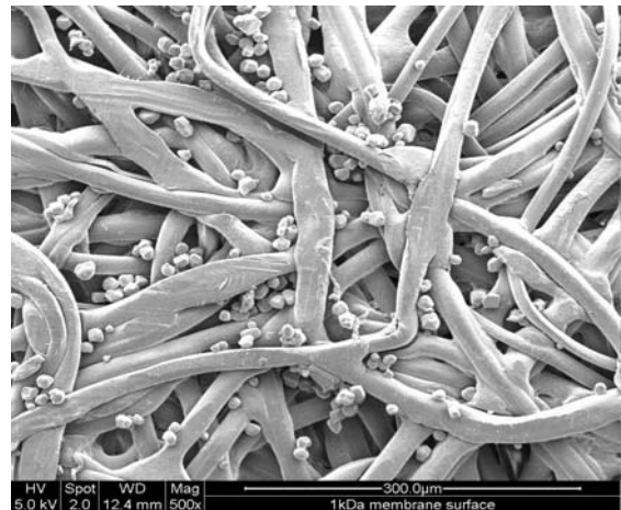
Fig. 14 SEM image of the surface of regenerated cellulose 1kDa membrane under 500 x magnifications
