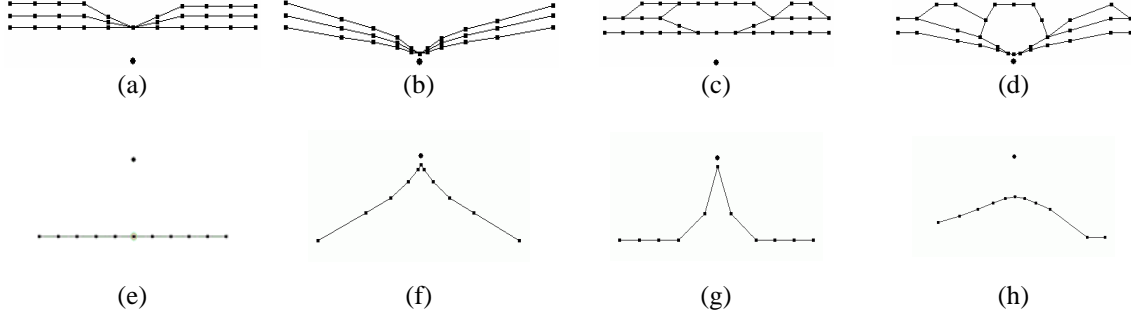
Fig. 1 A single iteration of SOM algorithm with different radius r and learning rate \alpha , on interconnected routes. (a)(c)(e) Initial configurations. (b)(d) r = 4, \alpha = 0.75 . (f) r = 4, \alpha = 0.9 . (g) r = 1, \alpha = 0.9 . (h) With asymmetric neighborhood r = 5;3, \alpha = 0.5
