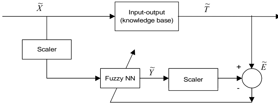
Fig. 2 Neural identification system
