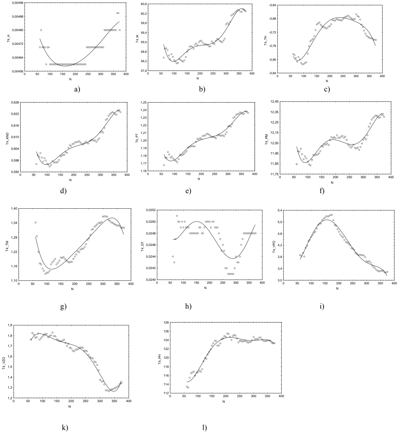
Fig. 6 Change of regression coefficient's values (influence) of parameters included in linear multiple regression equation D = (T_4^*)_{act} to T_4^* in GTE operation: a) T4_H – influence H on T_4^* (coefficient a'_1 ); b) T4_M – influence M on T_4^* (coefficient a'_2 ); c) T4_TH – influence T_H on T_4^* (coefficient a'_3 ); d) T4_KND – influence n_{LP} on T_4^* (coefficient a'_4 ); e) T4_PT – influence p_T on T_4^* (coefficient a'_5 ); f) T4_PM – influence p_M on T_4^* (coefficient a'_6 ); g) T4_TM – influence T_M on T_4^* (coefficient a'_7 ); h) T4_GT – influence G_T on T_4^* (coefficient a'_8 ); i) T4_VPO – influence V_{FS} on T_4^* (coefficient a'_9 ); j) T4_VZO – influence V_{BS} on T_4^* (coefficient a'_{10} ); k) T4_PH – influence p_H on T_4^* (coefficient a'_{11} ); N -number of measurements
