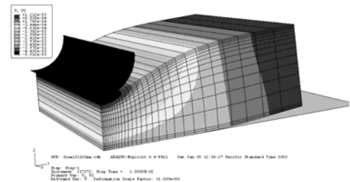
Fig 13 Indentation modeling of sandwich beam in Abaqus
