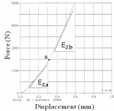
Fig. 3 Lateral compression in 4layer composite laminate
