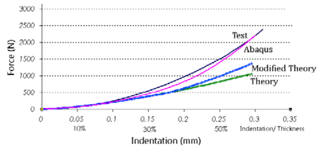
Fig. 9 Indentation in 2layer laminate with 10 mm indentor
