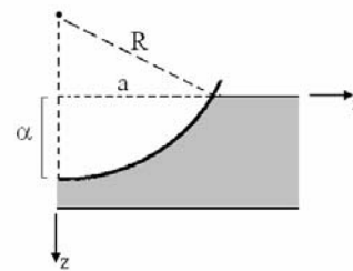
Fig. 4 Indentation of composite laminated
