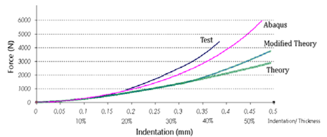
Fig. 10 Indentation in 4layer laminates with 20 mm indentor
