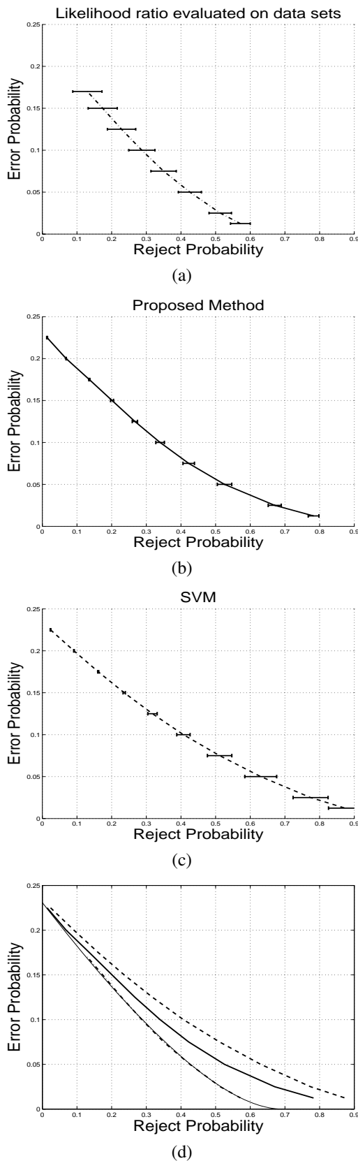
Fig. 8. Error-Reject curves (mean and standard-deviation bars) evaluated on 50 sets of 200 samples (a) using the true likelihood ratio evaluated o data sets, (b)using the proposed method, (c) using the SVM based method. In (d) the previous curves and the theoretical error-reject curve is also represented (solid), are represented all together for comparison
