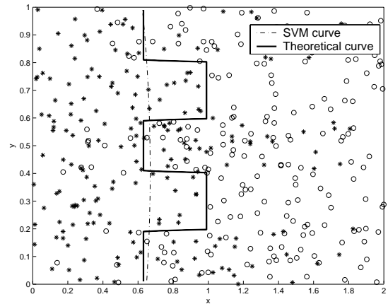
Fig. 6. Partitions corresponding to FPR= 0.1.
