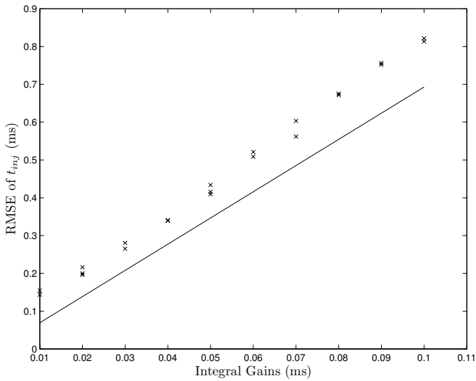
Fig. 7. Effect of integral gain on oscillation amplitude, measured by the standard deviation of 60 seconds of idling at each data point. The integral gains are symmetric ( K_{il} = -K_{ir} = K_i ). These values may be compared to the theoretical value from (6), shown as the solid line.
