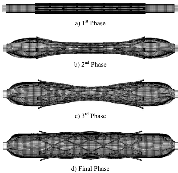
Fig. 1 The pattern of the transient non-uniform balloon-stent expansion at four different instants during the expansion process
