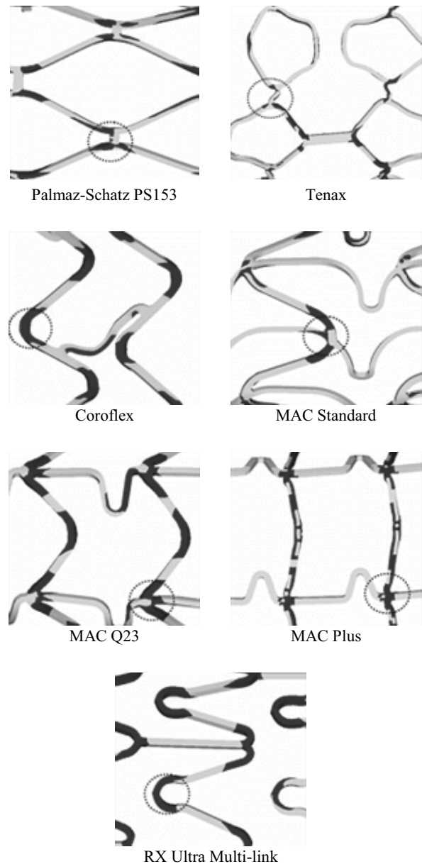
Fig. 2 Results of fatigue analysis (After 10 years)
