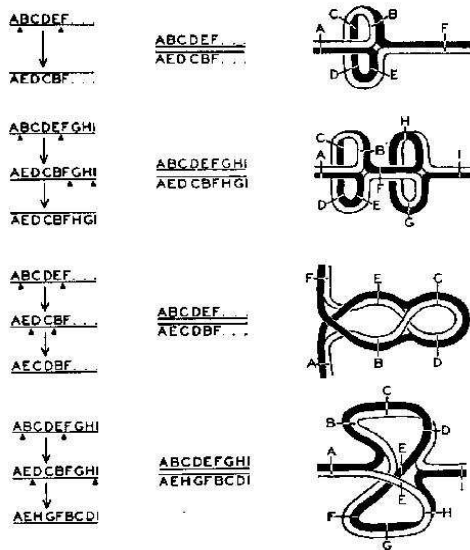
Fig. 2. Genome Rearrangements [12]
