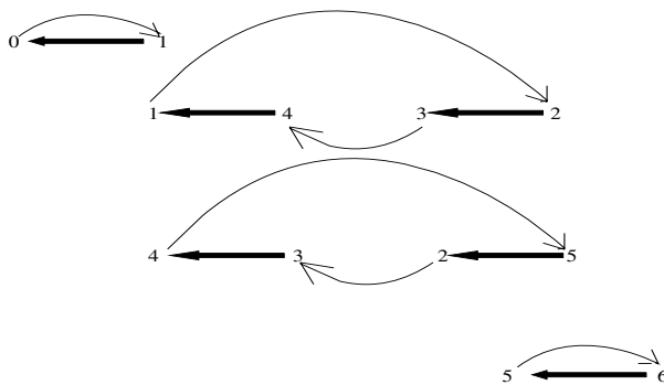
Fig. 5. Alternating cycles
