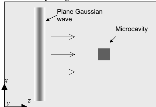
Fig. 1 The schematic arrangement showing a Gaussian plane wave launched into a microcavity consisting of 9 \times 9 TLM cells.
