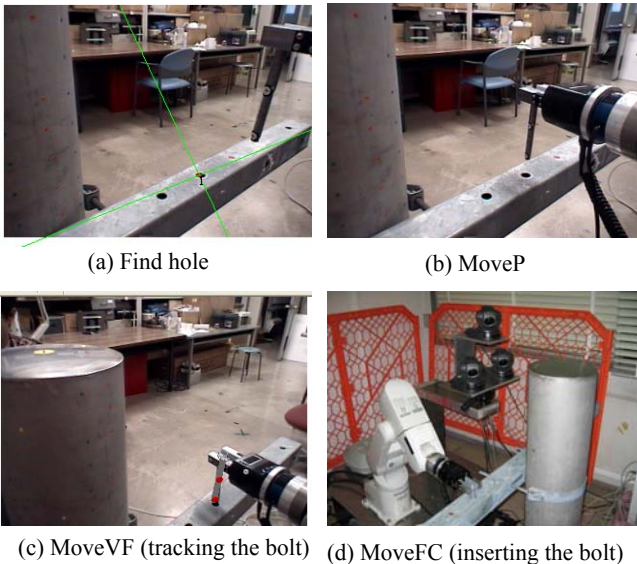
Fig. 9 The result of bolt insertion experiment
