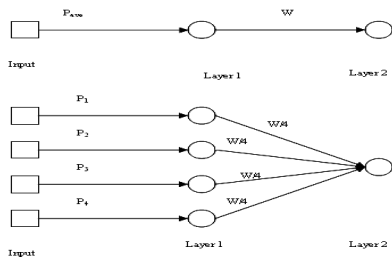
Fig. 6 Original neural network (top) and the “boosted” neural network (bottom)
