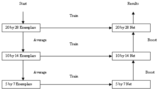
Fig. 5 Conceptual diagram of multiscale training technique
