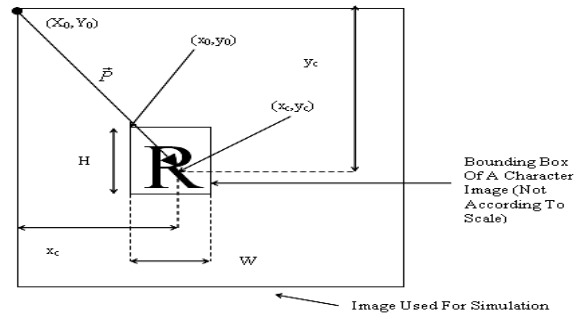
Fig. 7 The parameters used for character reassembly. Bounding box is defined with the width, w , height, h , horizontal centroid distance, x_c , vertical centroid distance, y_c , and vector that locates the centroid of a character from origin (X_0, Y_0), \vec{P}
