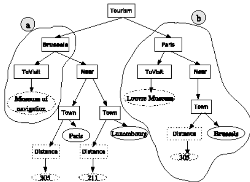
Fig. 7 Keyword Proximity
