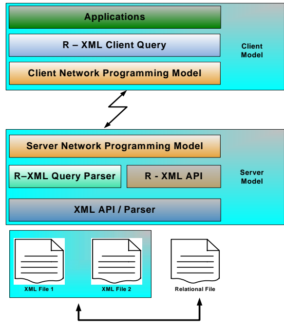
Fig. 9 R-XML Architecture
