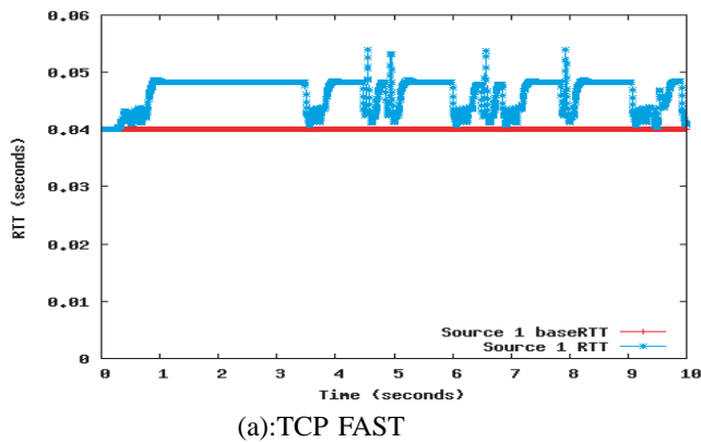
Fig. 15. Source 1 RTT variation with FAST TCP and VFAST TCP: scenario IV.
