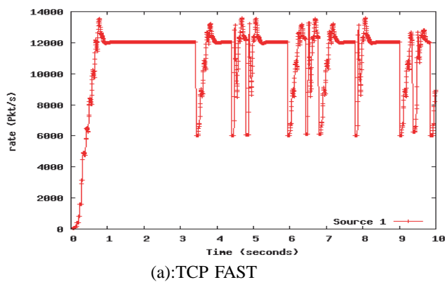
Fig. 16. Transmission rate variation of source 1 with FAST TCP and VFAST TCP: scenario IV.
