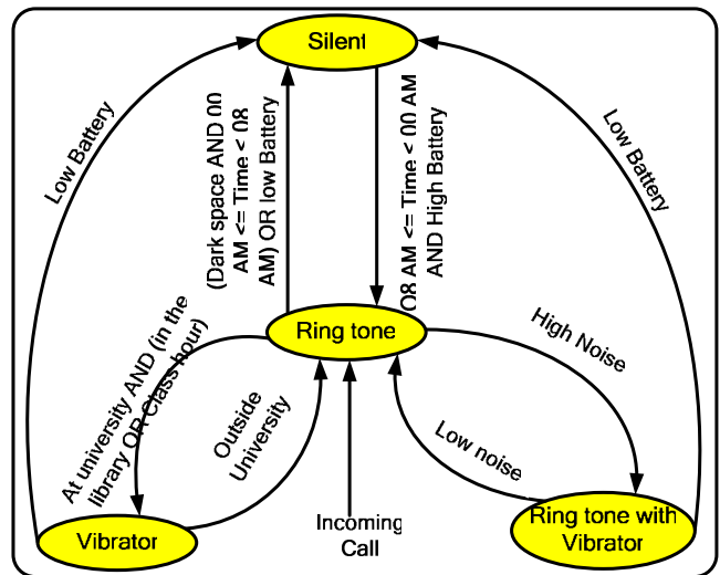
Fig. 4 Transition diagram of the application scenario
