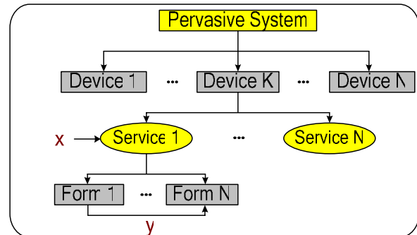
Fig. 1 Components of a pervasive system: The change in value of x_i will trigger service1. The change in value of y_j will change the form of service.
