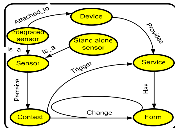
Fig. 2 Classes of the service ontology
