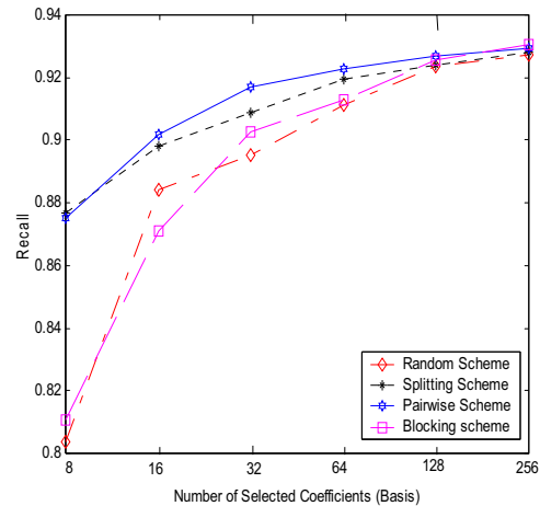
Figure 2: Recall vs. Various Axial Projection Options.
