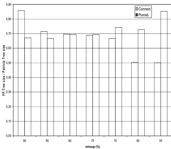
FIG 6. FP-TREE SIZE/PATRICIA-TREE SIZE FOR REAL DATASETS.
