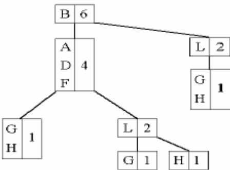
FIG 2. PATRICIA-TREE FOR DATASET D
