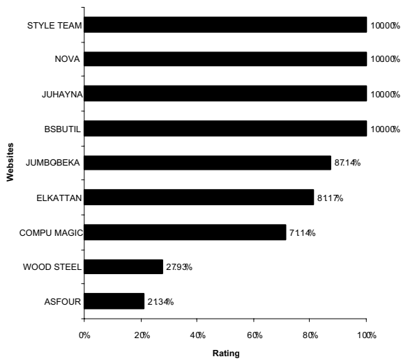
Fig. 3 Efficiency Scores
