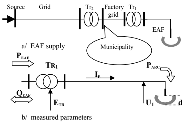
Fig. 3 Studied model
