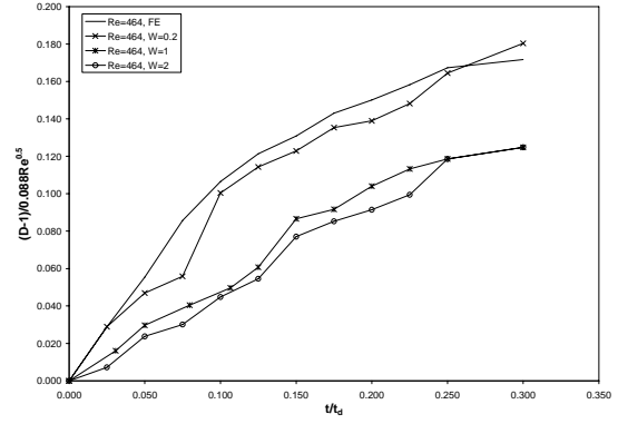
Fig. 5 Normalized fractal dimension of heavy particle lines as a function of the normalized time for k_N/k_1=100 and different particle drift velocities
