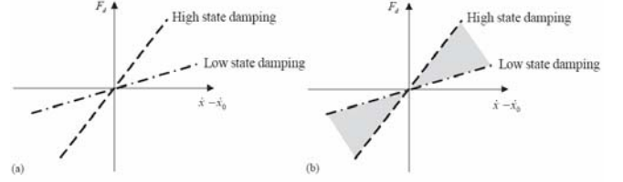
Fig. 2 Semi-active damper concepts
