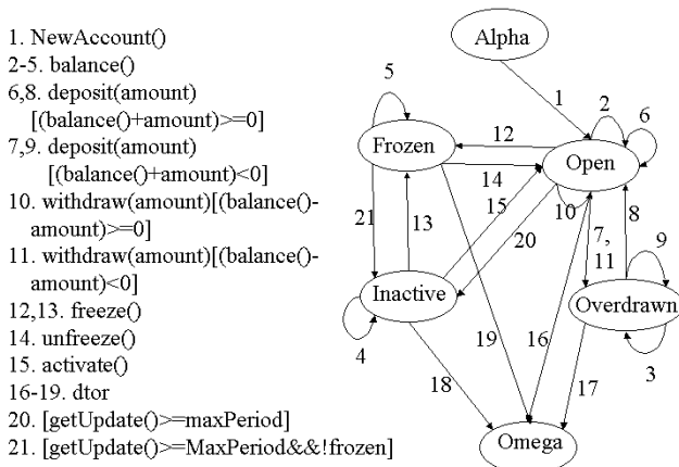
Fig. 2 The STD of the NewAccount object defined in the banking framework hooks.
