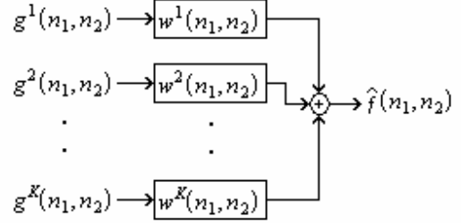
Fig. 2 Reconstruction stage
