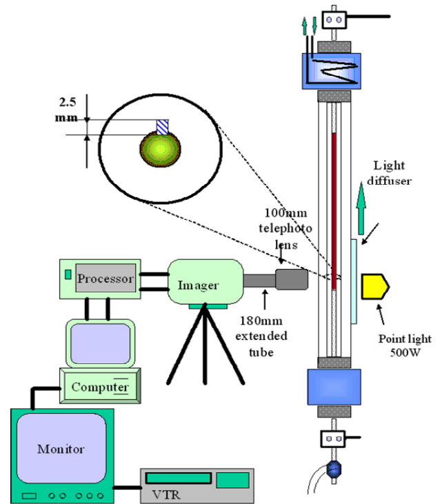
Fig. 4 Experimental setup of high speed photography
