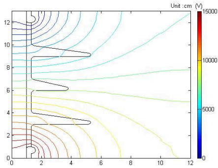
(b) Alternate Sheds Insulator
