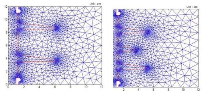
(a) Straight Sheds insulator (b) Alternate Sheds Insulators Fig. 6 Finite element discretization results
