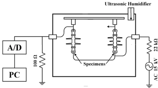
Fig. 2 Test Arrangement
