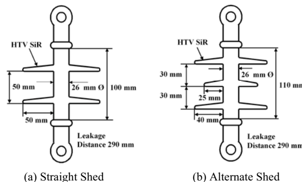
Fig. 1 Test Specimens
