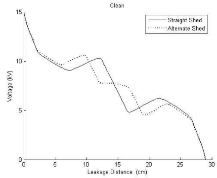
Fig. 9 Comparison of Potential Distribution
