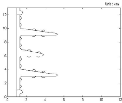
Fig. 12 Alternate Sheds Insulator with Water Droplets on the Surface
