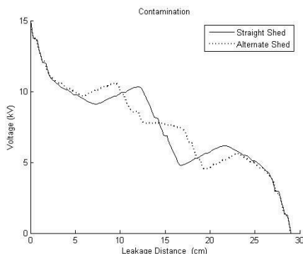
Fig. 14 Comparison of Potential Distribution under Contamination Condition
