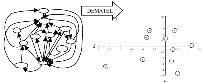
Fig. 5 DEMATEL method
