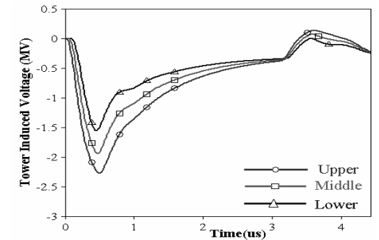
(c) Lightning Stroke Current Waveform 2.0/77.5 \mu s
