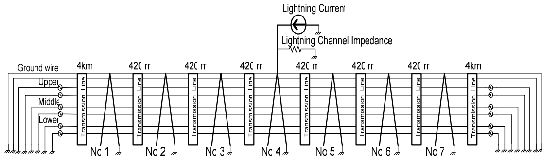
Fig. 3 Span of 7 Towers in This Study
