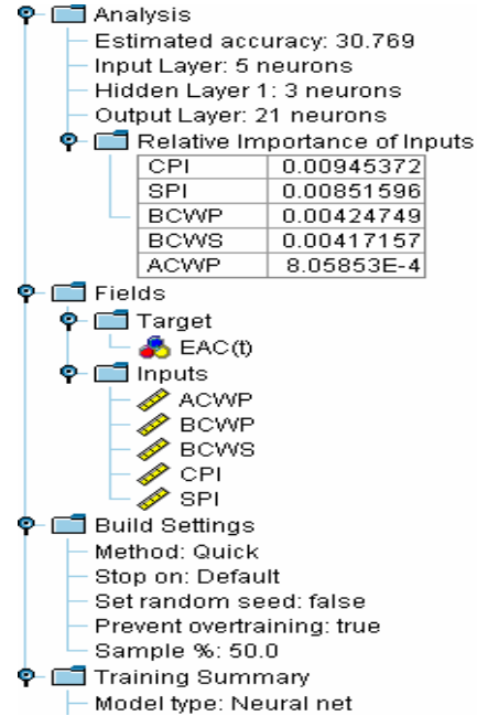
Fig. 4 Neural Network
