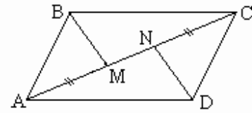
Fig. 2 Problem: prove that \Delta ABM = \Delta CDN
