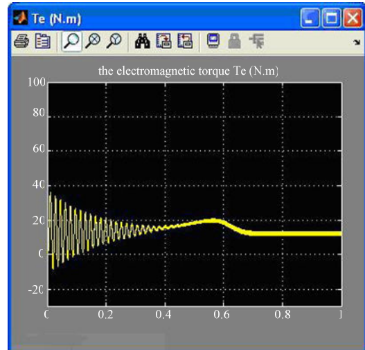
Fig. 10 Time Response of electromagnetic torque of induction motor
