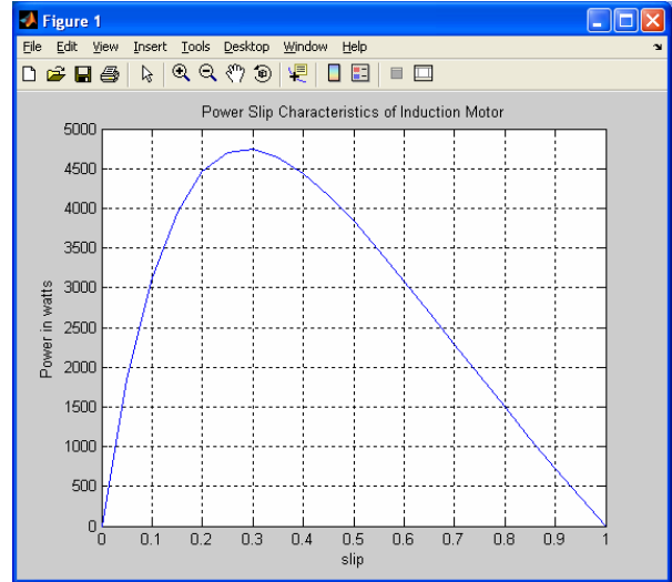
Fig. 3 Power slip characteristic of induction motor
