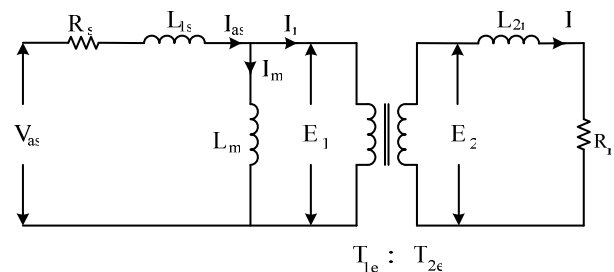
Fig. 1 Elementary equivalent circuit for induction motor
