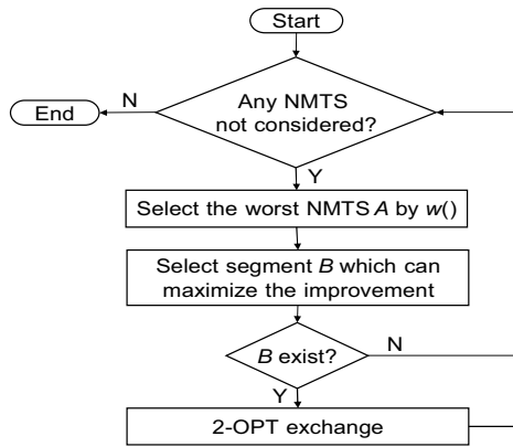
Fig. 11 The flowchart of the intelligent OPT
