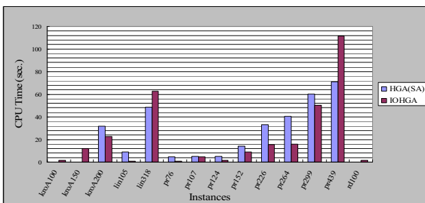
Fig. 16 The CPU time
