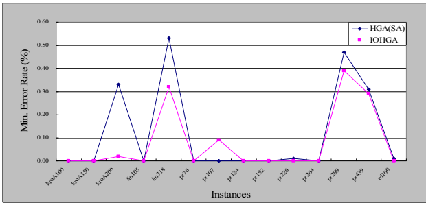
Fig. 12 The minimal error rates
