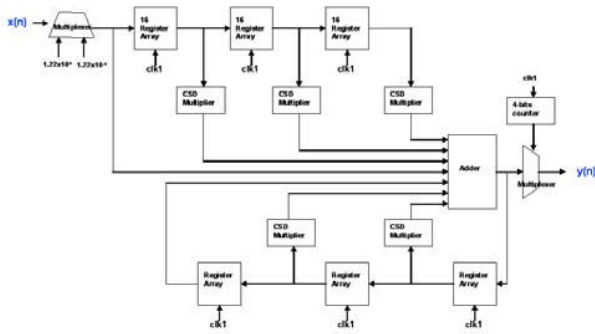
Fig. 8 CIC filter implementation using polynomial expansion
