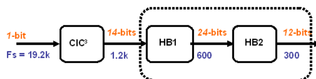
Fig. 1 Building blocks of a decimator filter
