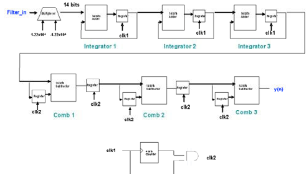
Fig. 6 CIC filter implementation using cascaded accumulator-differentiator approach
