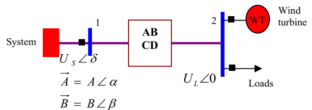
Fig. 4 Radial feeder with connected WG
