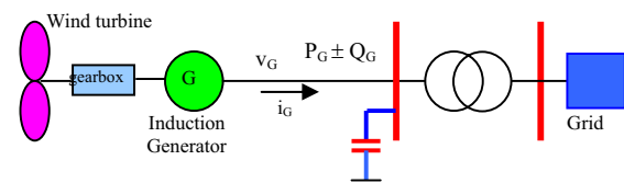
Fig. 1 Modelling wind turbine connected grid [1]
