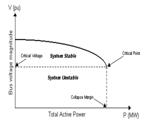
Fig. 2 Charactic P-V
