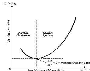
Fig. 3 Charactic Q-V
