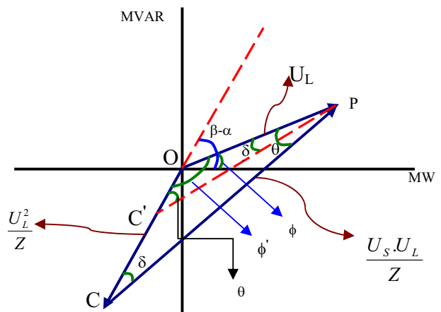
Fig. 6 UPCD for short distribution line
