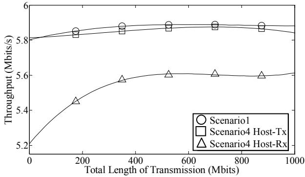
Fig. 8 Throughput for scenario 4
