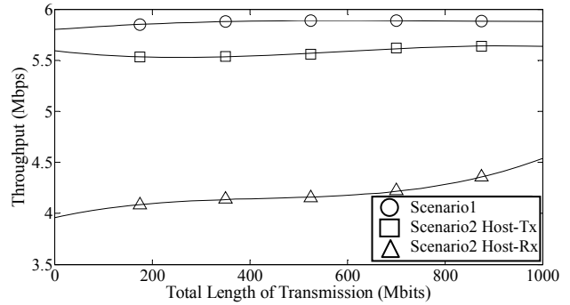
Fig. 4 Throughput, Scenario 1 Vs Scenario 2
