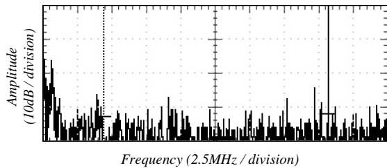
Fig. 15 Spectral Plot for the Background Generalized Noise. Spam 25MHz, Center 12.5MHz, Reference -47dB
