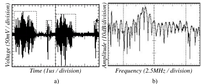
Fig. 11 Impulsive noise measured for scenario 2
