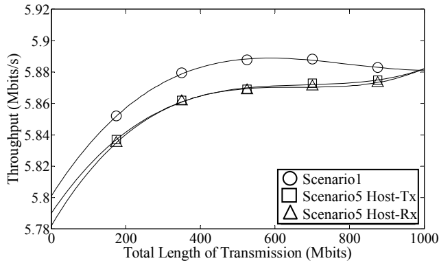
Fig. 9 Throughput for Scenario5
