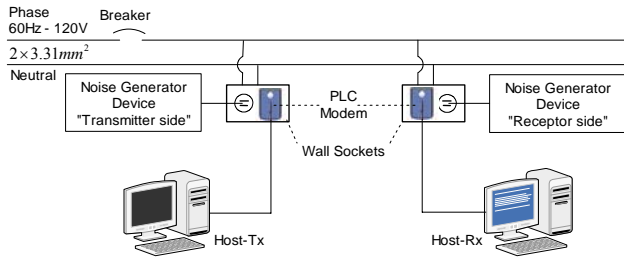
Fig. 3 Basic Networking Model
