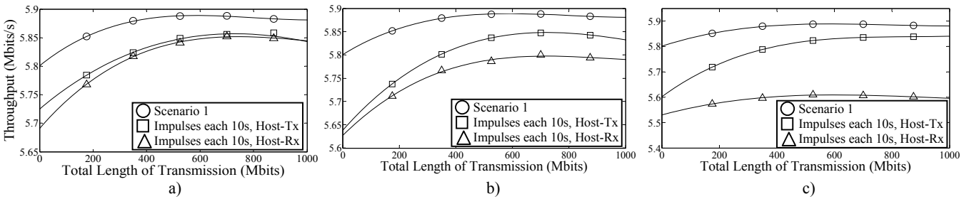
Fig. 6 Throughput for scenario3 for astable period times of a) 10sg, b) 5sg, c) 2.5sg
