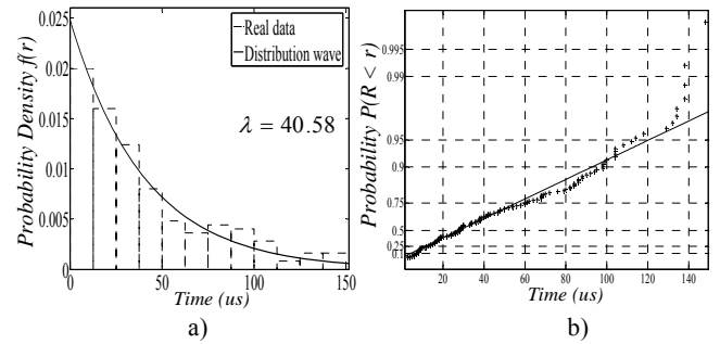
Fig. 14 Exponential function distribution for inter-arrival times a) PDF b) Exponential probability
