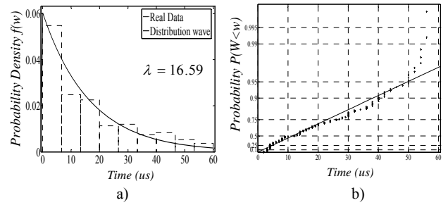
Fig. 13 Exponential function for the impulses duration a) PDF b) Distribution Function
