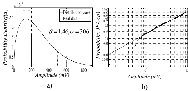
Fig. 12 Weibull Distribution a) PDF, b) Amplitude function
