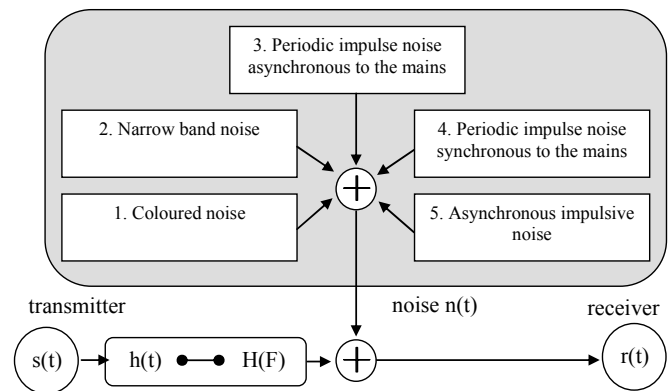
Fig. 2 Classification of Noise on PLC Channels
