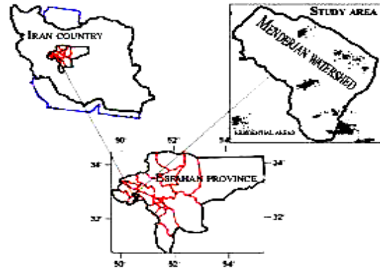
Fig. 1 Position of study area in Esfahan province and Iran country
