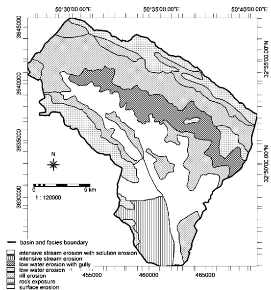
Fig. 2 Erosion forms map of study area
