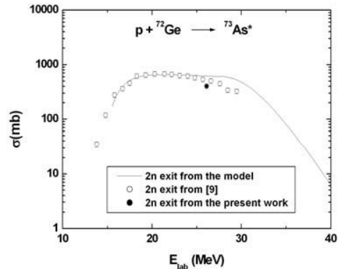
Fig. 6 Solid line refers to the cross sections for ^{72}\text{Ge}(p,2n)^{71}\text{As} estimated by the compound nucleus reaction model. Open symbols refer to the data from [9] and the closed one to the present work.
